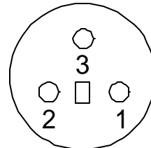
FEMALE SOCKET END VIEW
